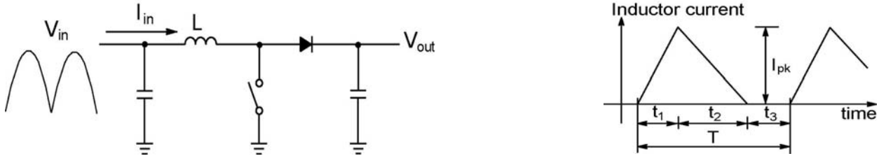
Figure 64. PFC Boost Converter (left) and Inductor Current in DCM (right)
